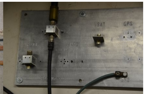
Lightning protection on the 7/8 inch Andrew LDF5-50A Heliex feedline... that aluminum mounting plate is 3/4 inch thick!
